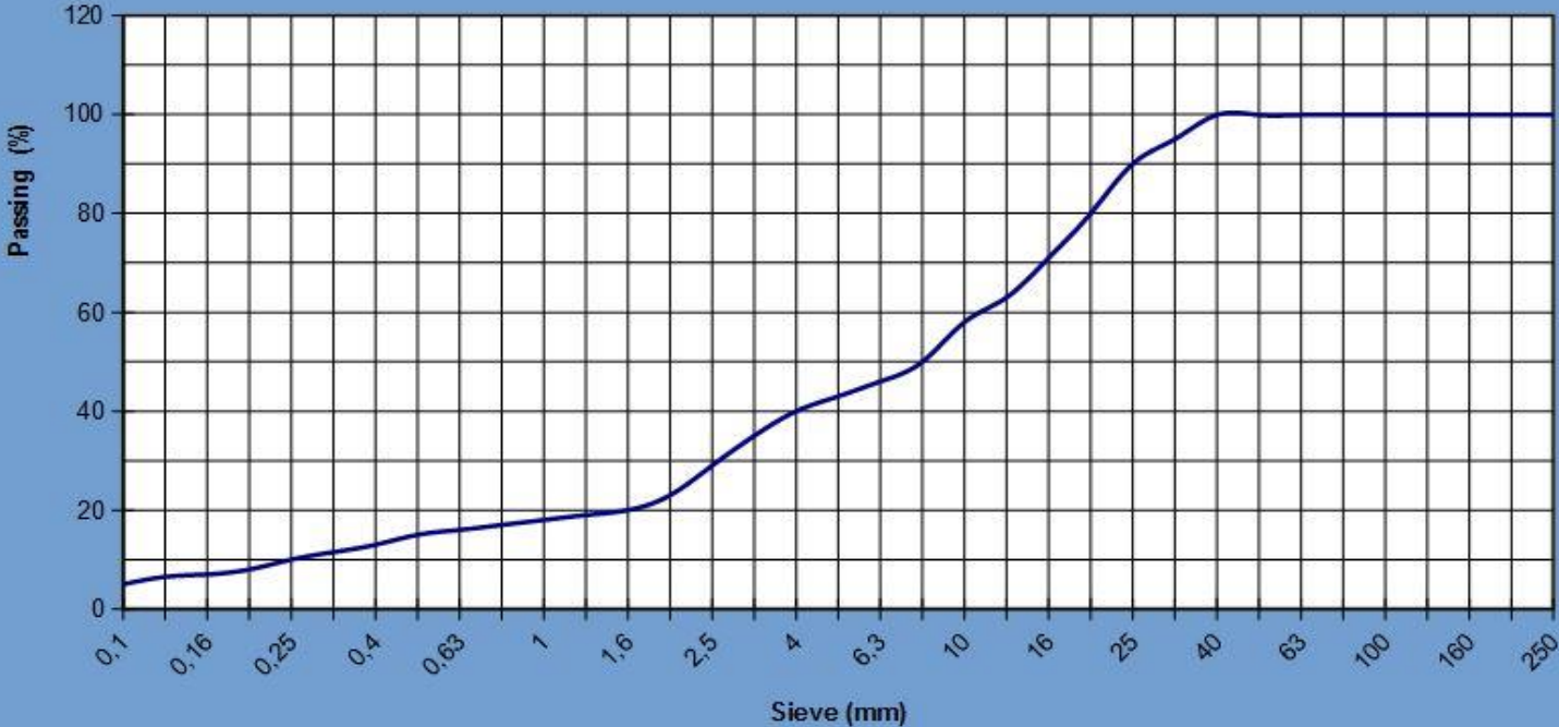
DRAGON 9 Material : Limestone Feeding size : 0 - 650 mm Rotor Speed : 36 m/sc Adjustment : 30 mm Capacity : 100-150 t/h
